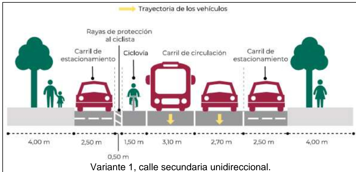
Figura 68.- Calles colectoras [1] [2] [3]
